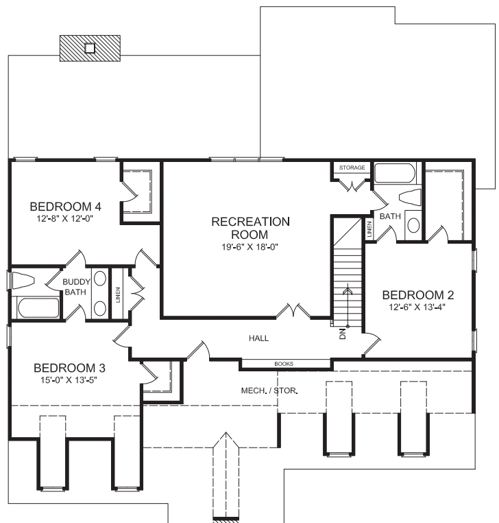
SECOND FLOOR
